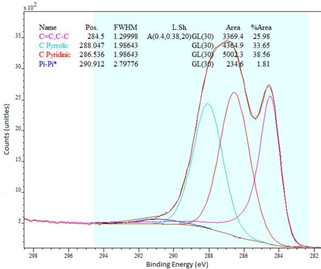
Figure 4-7: Representative C 1s XPS Spectra showing the binding energies for the four different carbon bonding configurations.
