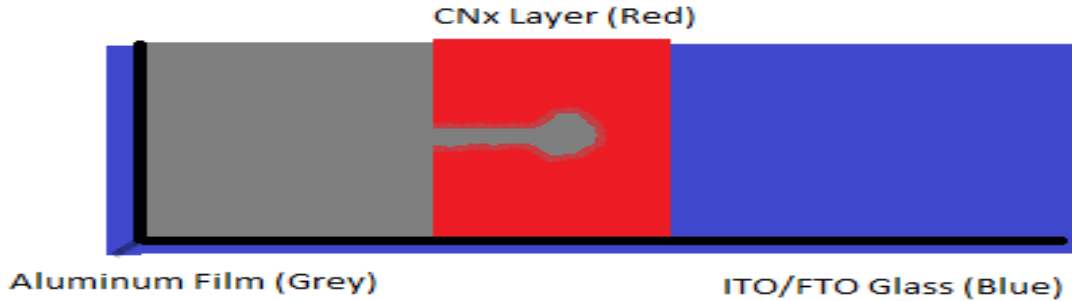
Figure 1-4: Schottky architecture used for prepared samples.
